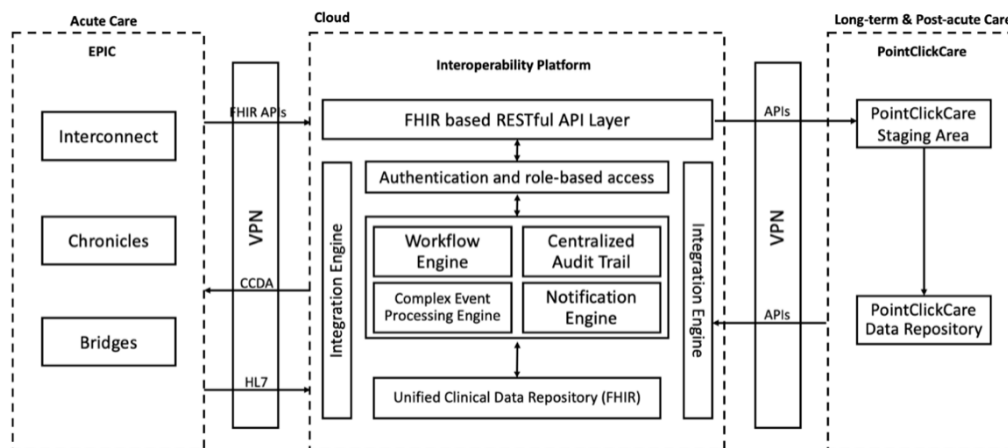
Figure 1: Interoperability Architecture for Information Exchange
